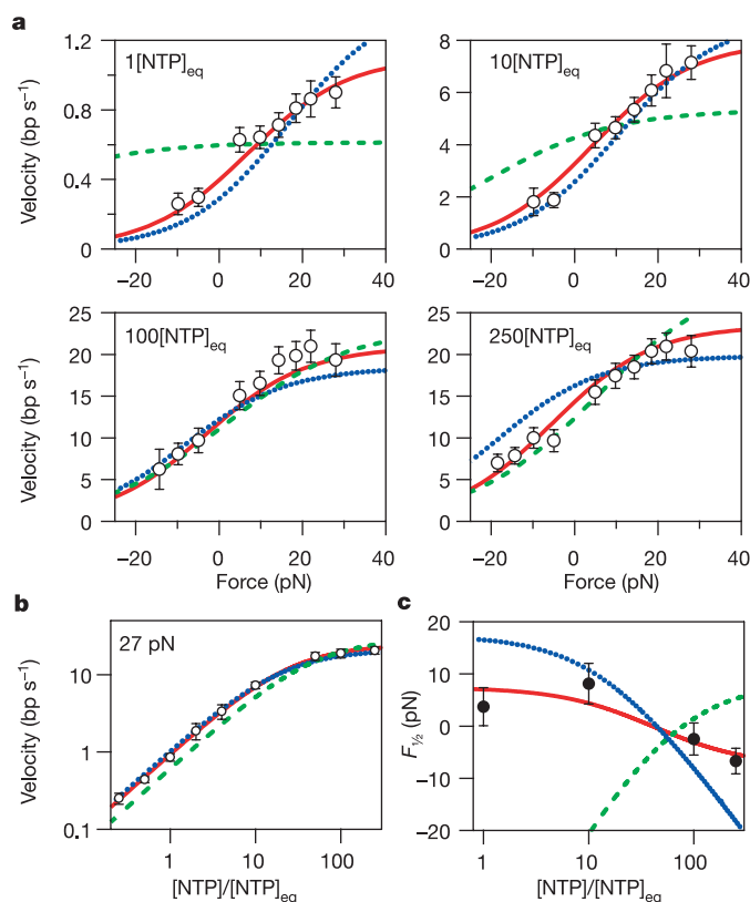
Figure 5 | Force-velocity and Michaelis-Menten relationships along with model fits. a , b , Measured force-velocity relationships for RNAP at [\text{NTP}]_{\text{eq}} , 10[\text{NTP}]_{\text{eq}} , 100[\text{NTP}]_{\text{eq}} and 250[\text{NTP}]_{\text{eq}} , with off-pathway events removed (see text) ( a ), and single-molecule velocity as a function of [\text{NTP}] measured at 27 pN assisting load (open circles) with associated errors (see Methods) ( b ). Negative forces correspond to hindering loads; positive forces to assisting loads. Global fits to the power stroke model of Fig. 3a (green dashed line), the brownian ratchet model of Fig. 3b (blue dotted line) and the Michaelis-Menten model of Fig. 3c (solid red line) are shown. c , The F_{1/2} value as a function of [\text{NTP}] derived from free fits of the data in a to equation (1) (Supplementary Fig. S4), shown together with predictions from the three models (coloured lines) (Supplementary Fig. S5).
